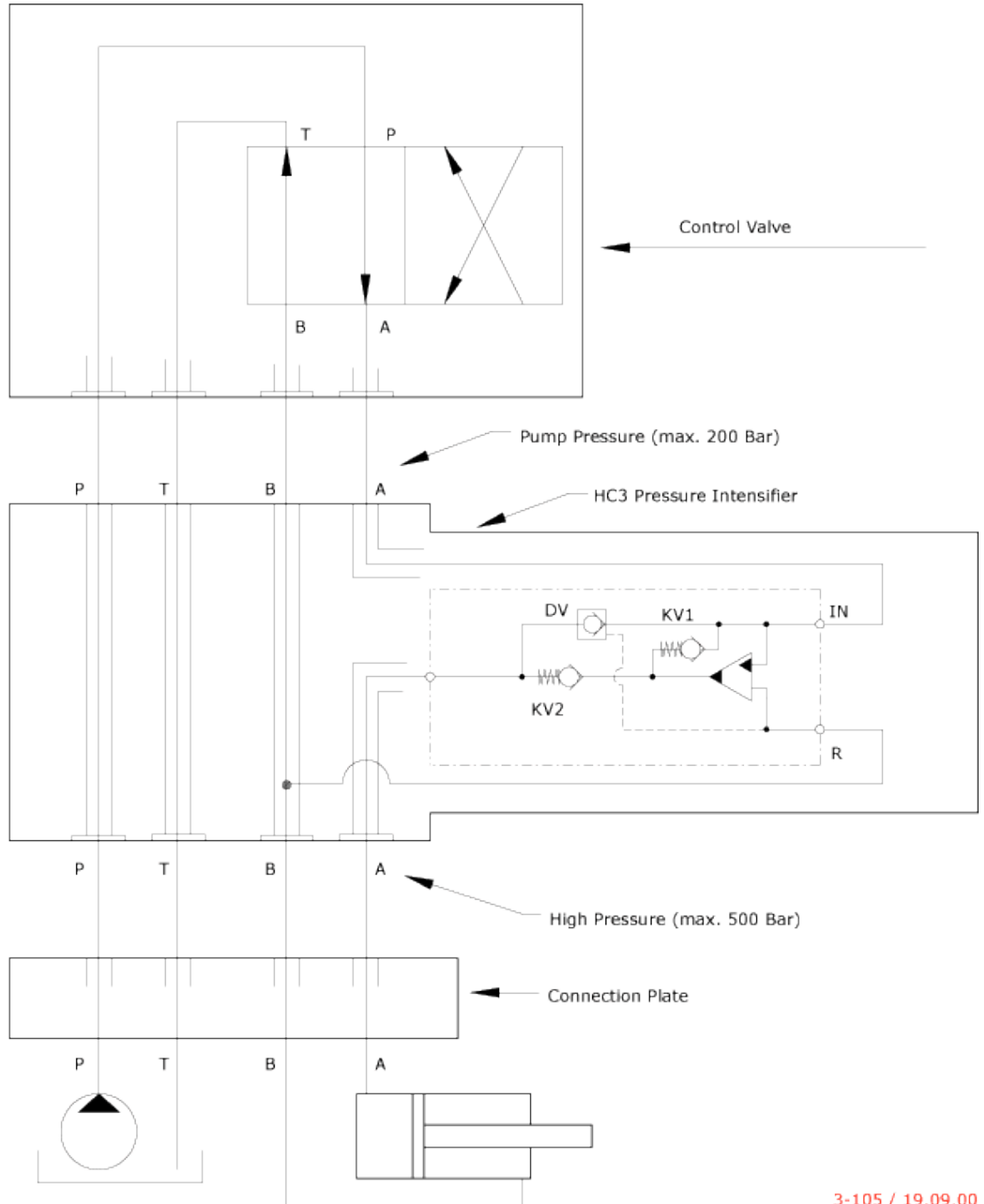
Function Diagram
