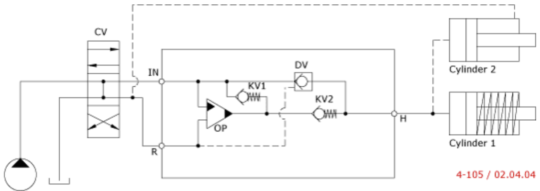
Function Diagram
