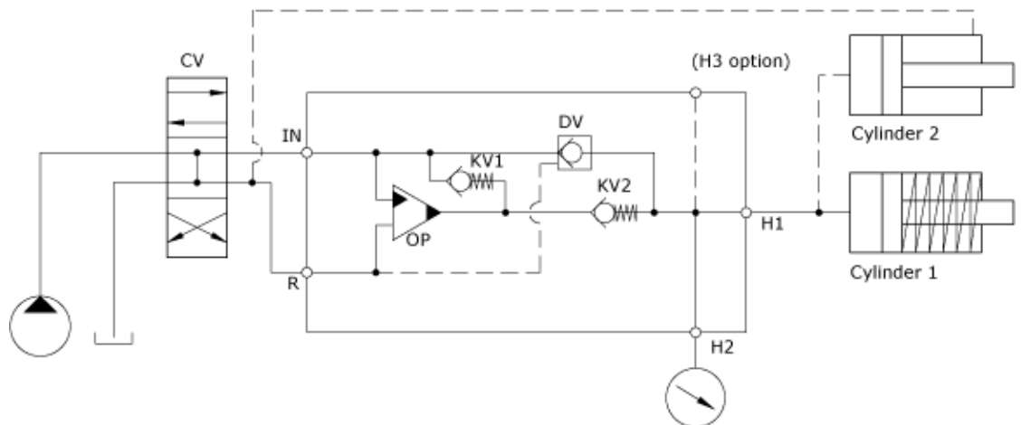
Function Diagram
